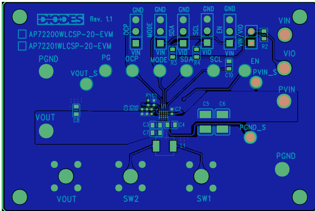
Figure 3. AP72200-EVM – Top Layer
