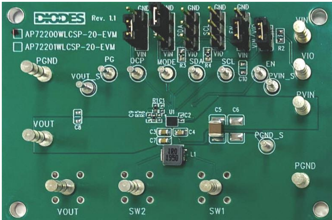
Figure 1. AP72200-EVM
