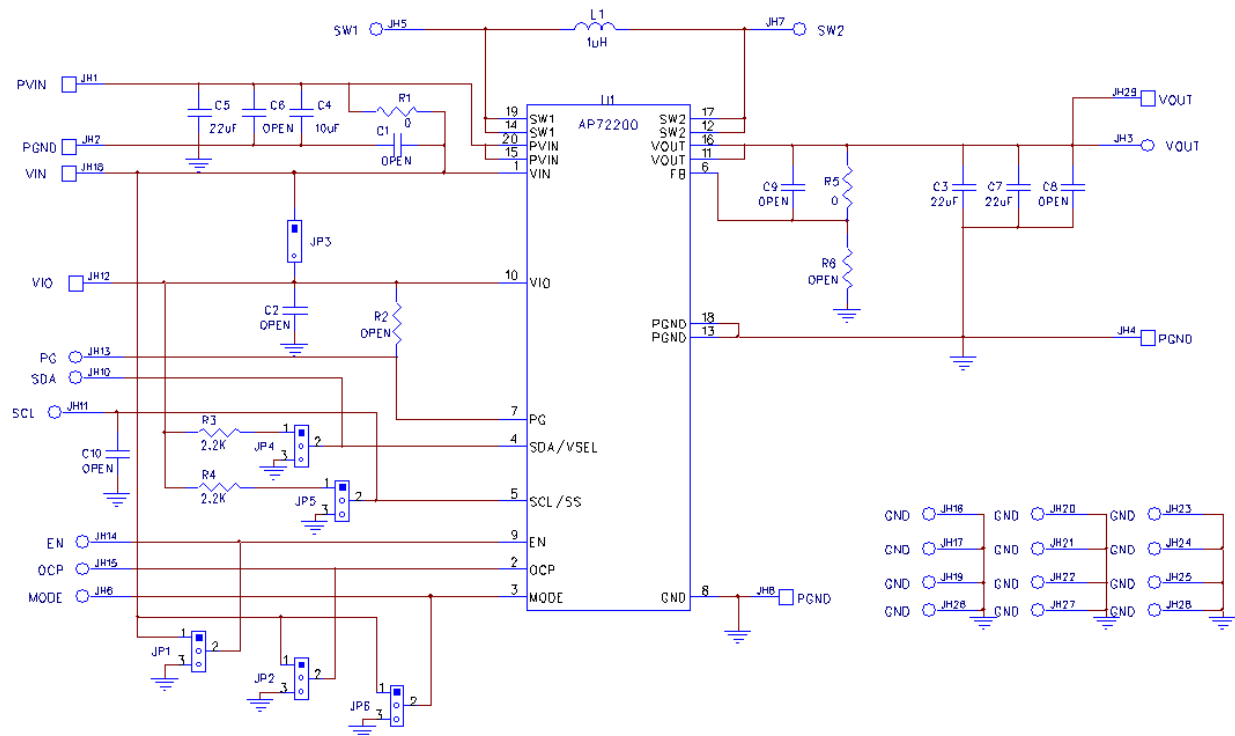
Figure 2. AP72200-EVB Schematics
