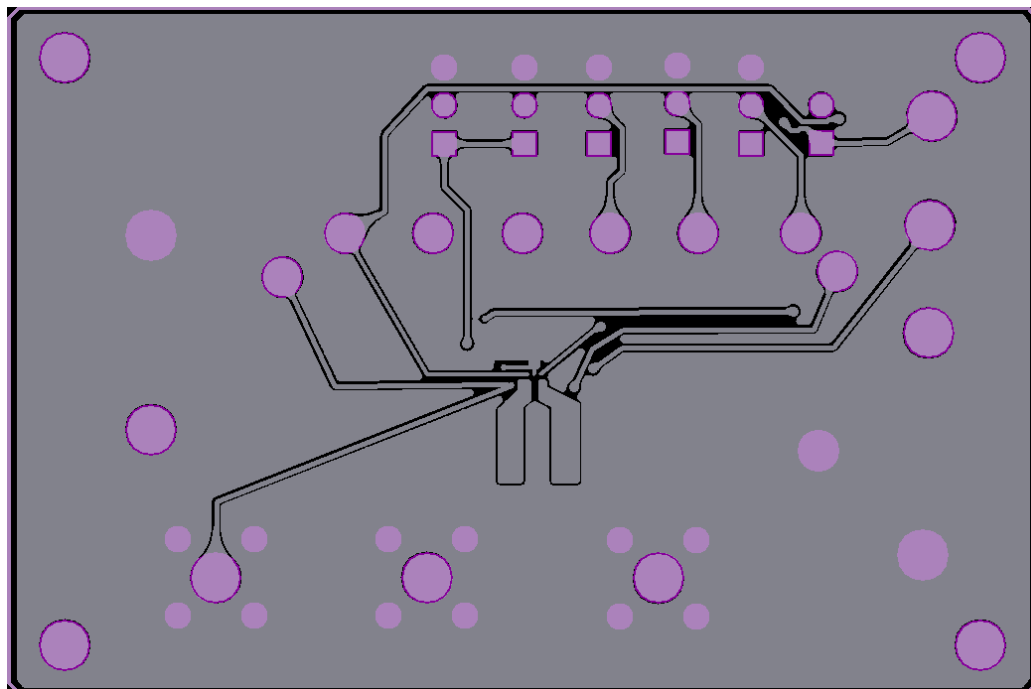
Figure 4. AP72200-EVM – Bottom Layer
