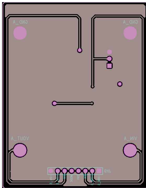
Figure 4. AP64060QWU-EVB – Bottom Layer
