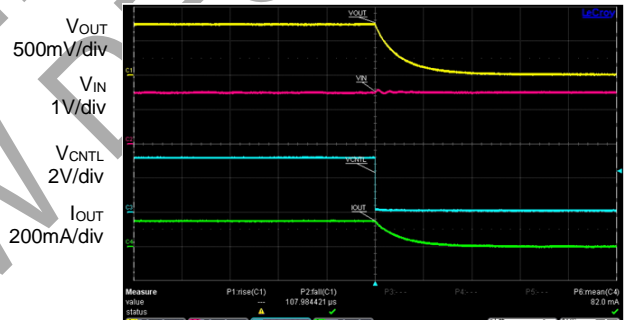
Time 100µs/div
